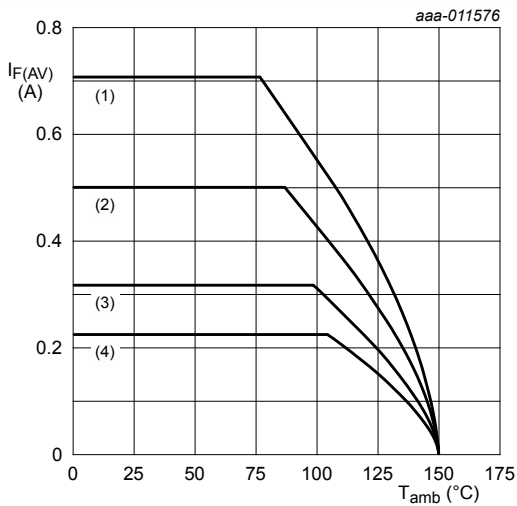
FR4 PCB, mounting pad for anode and cathode 1 \text{cm}^2 each T_j = 150\text{ }^\circ\text{C} (1) \delta = 1 ; DC (2) \delta = 0.5 ; f = 20\text{ kHz} (3) \delta = 0.2 ; f = 20\text{ kHz} (4) \delta = 0.1 ; f = 20\text{ kHz}
